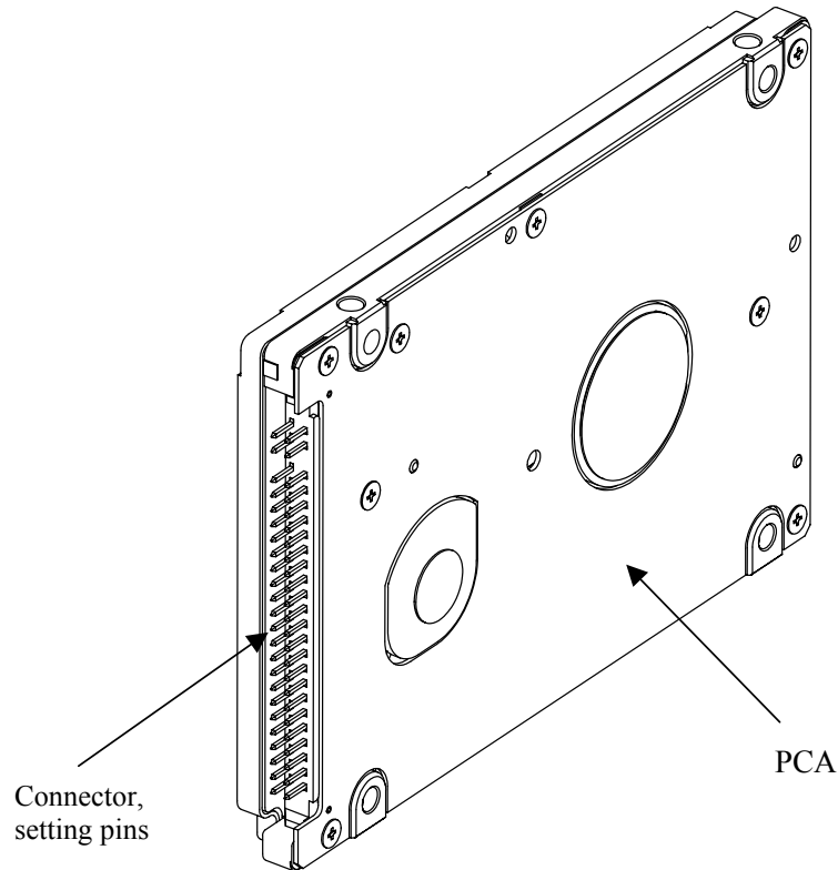
Figure 3.7 Connector locations
